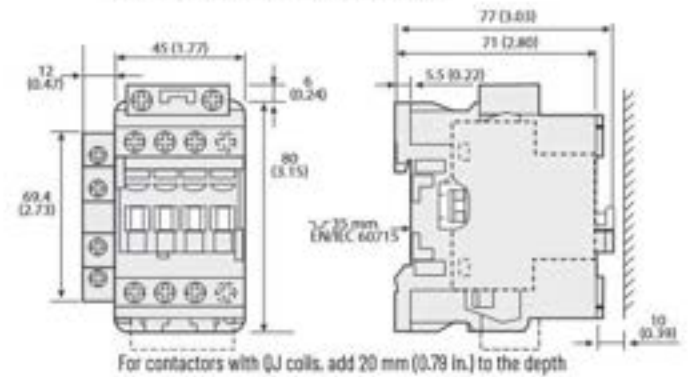
Figure 38 - 100-E09...100-E16 Contactors with Standard Coils and Side-mounted Auxiliary Contact
