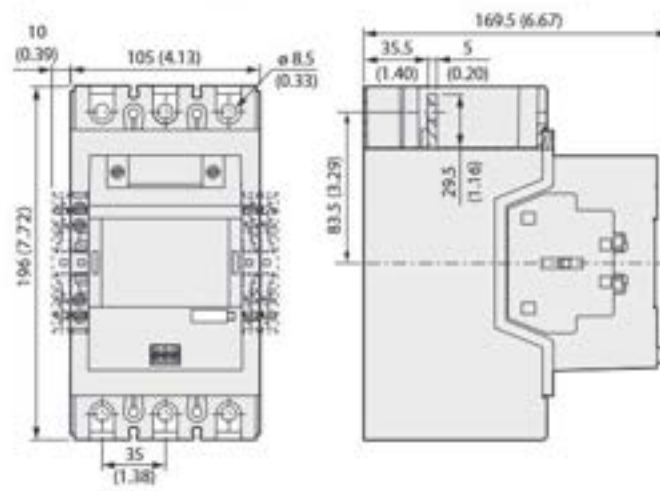
Figure 81 - 100-E190E, 100-E205E Contactors with PLC Input
