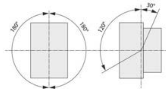
Figure 75 - Mounting Position for 100-E116...100-E2650 Devices— AC/DC and AC/DC with PLC input
