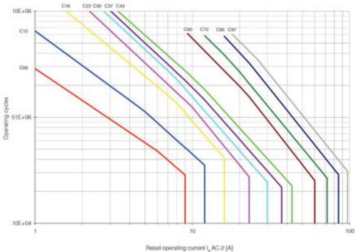
Figure 12 - AC-2, Switching of slip-ring motors; U_g = 230...400...460V
