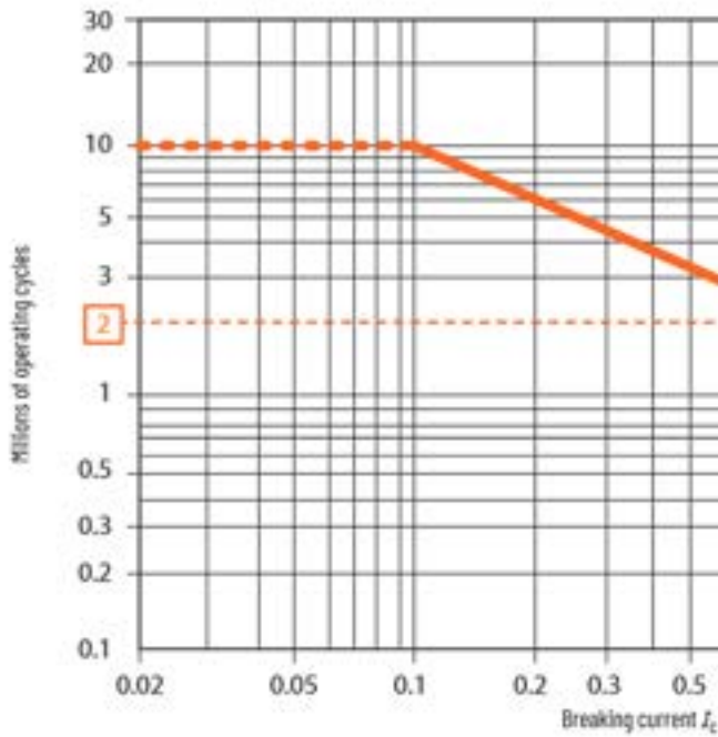
Figure 32 - Electrical durability for DC-13 utilization category - U_e \leq 250V
