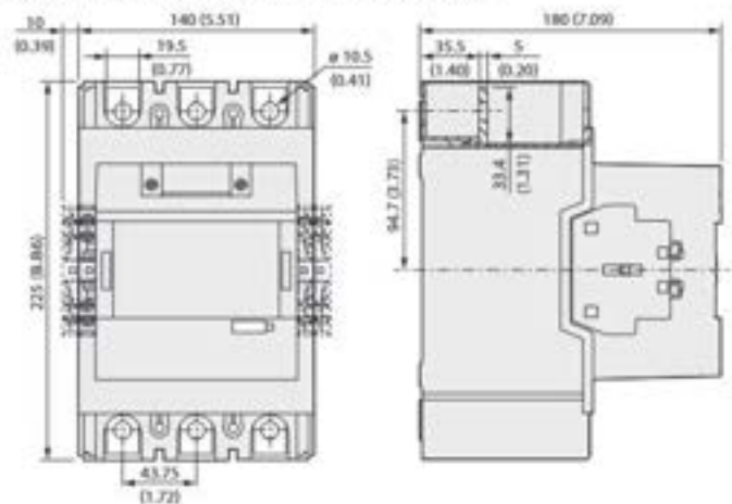
Figure 84 - 100-E265...100-E370 Contactors
