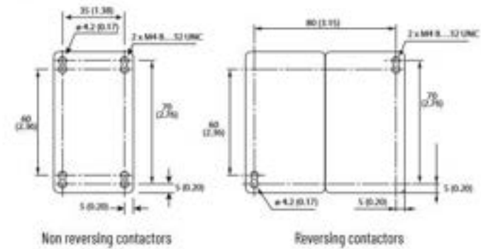
Figure 62 - 100-E40...100-E52 4-Pole Contactors
