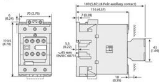
Figure 67 - 100-E80...100-E96 3-Pole Contactors with Front-mounted Auxiliary Contact
